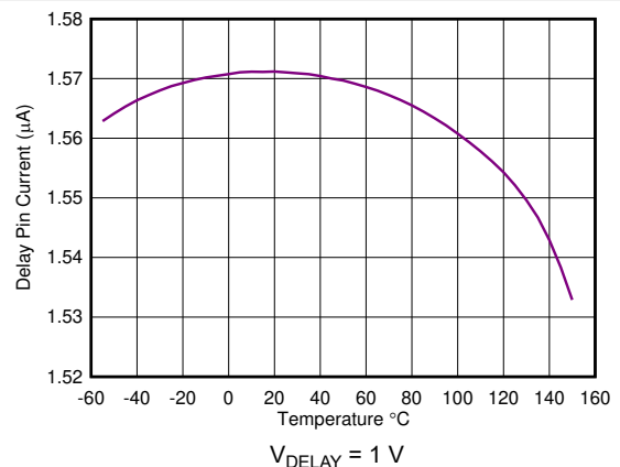
Figure 6-36. Delay Pin Current vs Temperature V_{DELAY} = 1\text{ V}
