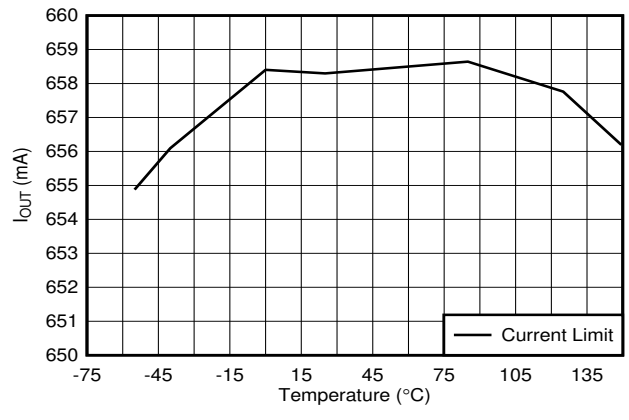
Figure 6-26. Output Current Limit vs Temperature
