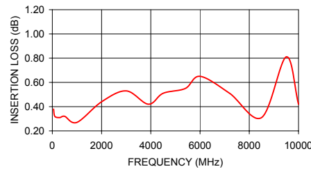
INSERTION LOSS
