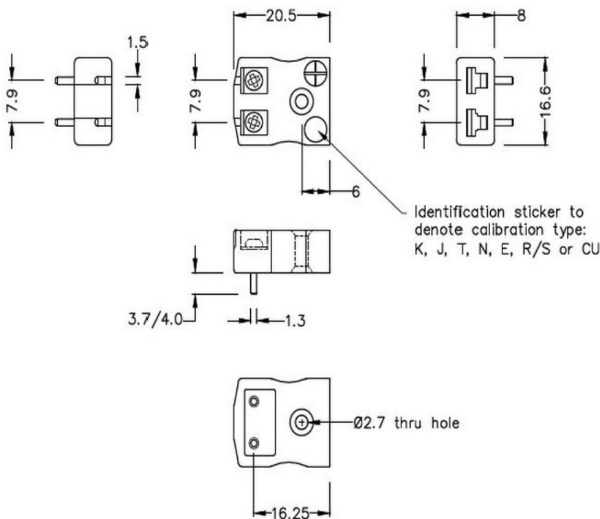
Miniature PCB Socket (dimensions in mm)
